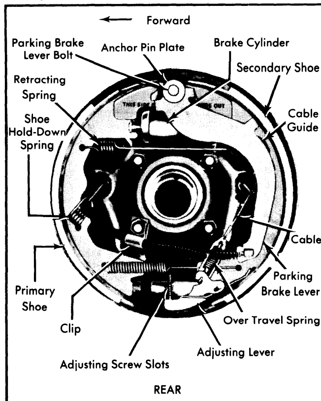
Fig. 4 Ford Motor Co. Rear Brake Assembly (250 and 350 Models)
