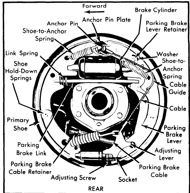
Fig. 3 Ford Motor Co. Rear Brake Assembly (100, 150 and Bronco Models)
