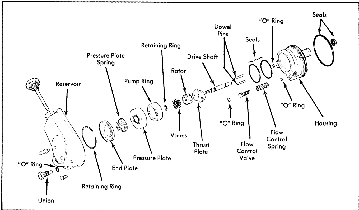
Fig. 6 Exploded View of Power Steering Pump
