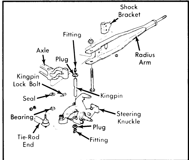
Fig. 4 Identification of Suspension Details "E" Models (Exc. E-250 and E-350 Steering Knuckle)
