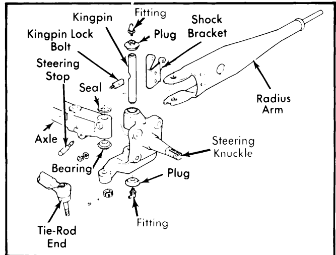
Fig. 5 Identification of Suspension Details E-250 and E-350 Steering Knuckle
