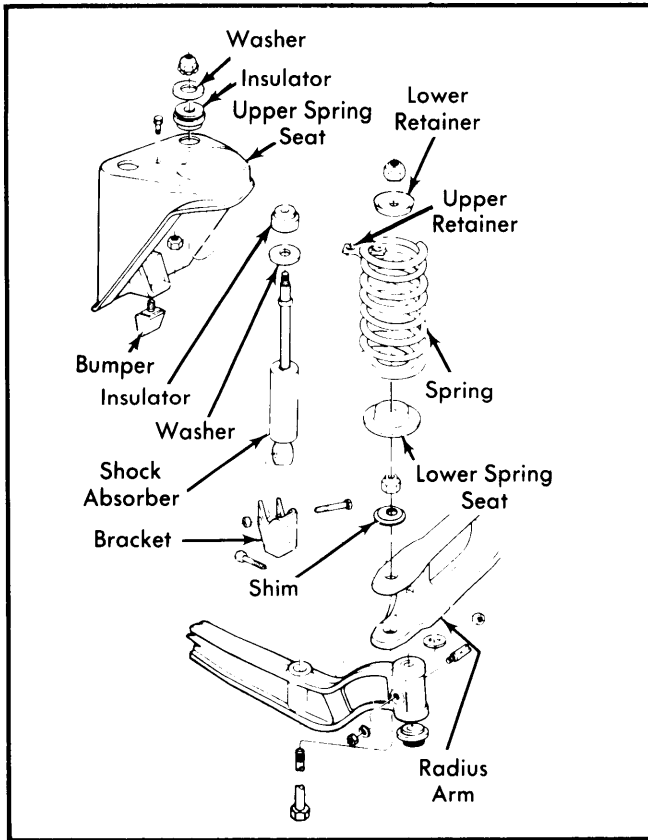
Fig. 3 Identification of Suspension Details F-100, 150 and 250 Shown, F-350 Similar
