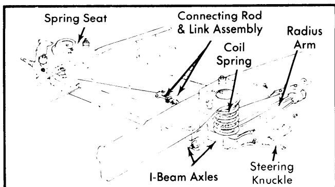
Fig. 1 Identification of Front Suspension Components F-100, F-150 and F-250, Under 6800 GVW (Others Similar)
