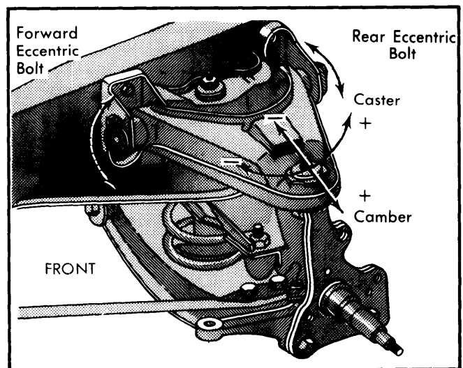
Fig. 2 Wheel Alignment Adjustments (AD, AW, D, PD, PW and W Models)
