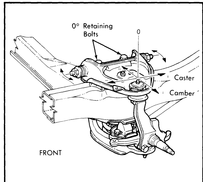
Fig. 3 Wheel Alignment Adjustments (B, CB, MB and PB Models)
