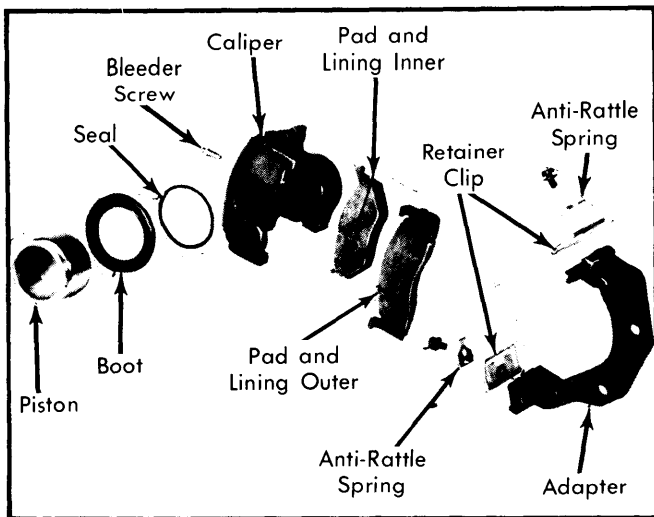
Fig. 1 Exploded View of Chrysler Single Piston Disc Brake Caliper
