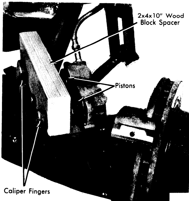
Fig. 6 Removing Caliper Pistons
