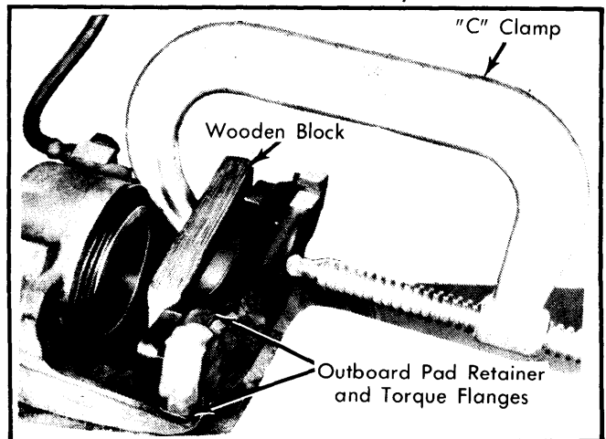
Fig. 4 Installation of Outboard Pad and Liner
