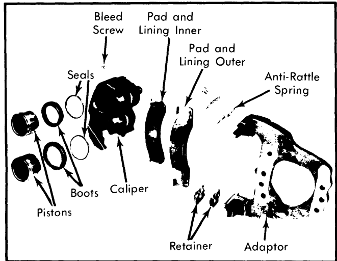
Fig. 3 Exploded View of Chrysler Two Piston Disc Brake Caliper
