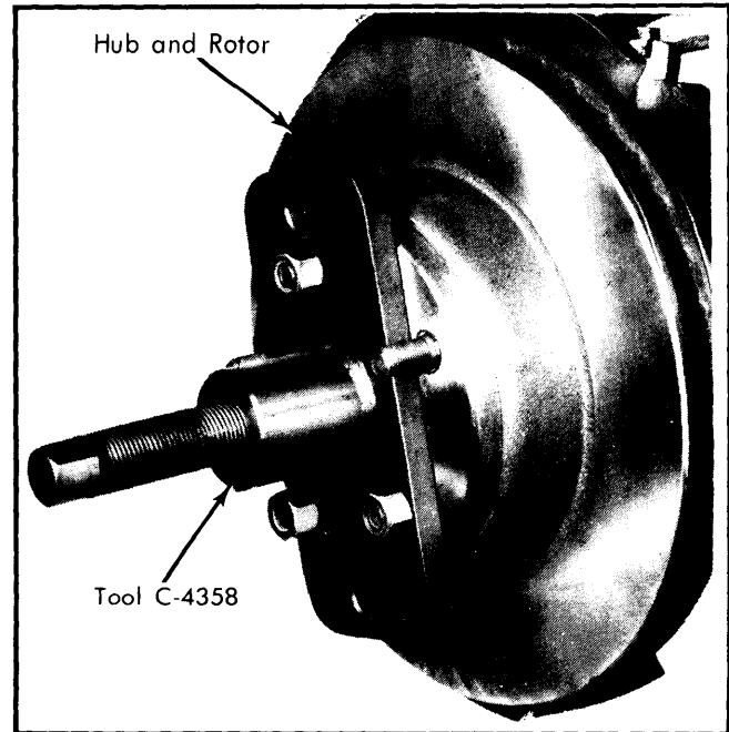
Fig. 5 Removing Rotor Hub (44FBJ Axle)
