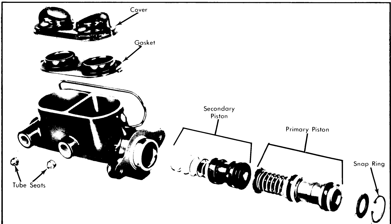
Fig. 2 Exploded View of Cast Iron Master Cylinder
