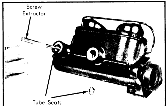
Fig. 1 Removing Tube Seats from Master Cylinder
