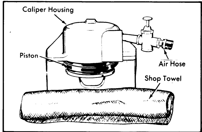
Fig. 2 Using Compressed Air to Remove Caliper Piston
