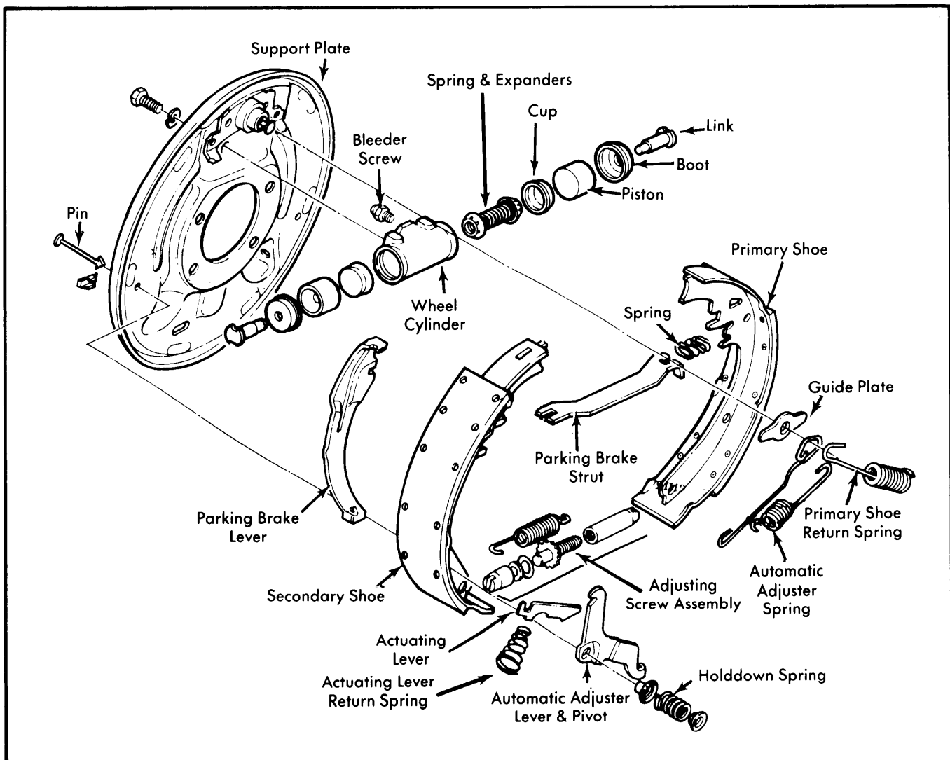
Fig. 1 Exploded View of Jeep Brake Assembly
