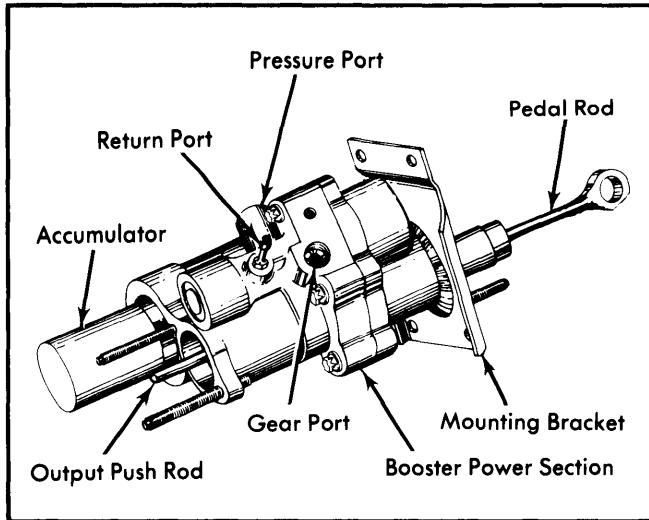
Fig. 7 Bendix Hydro-Boost Assembly
