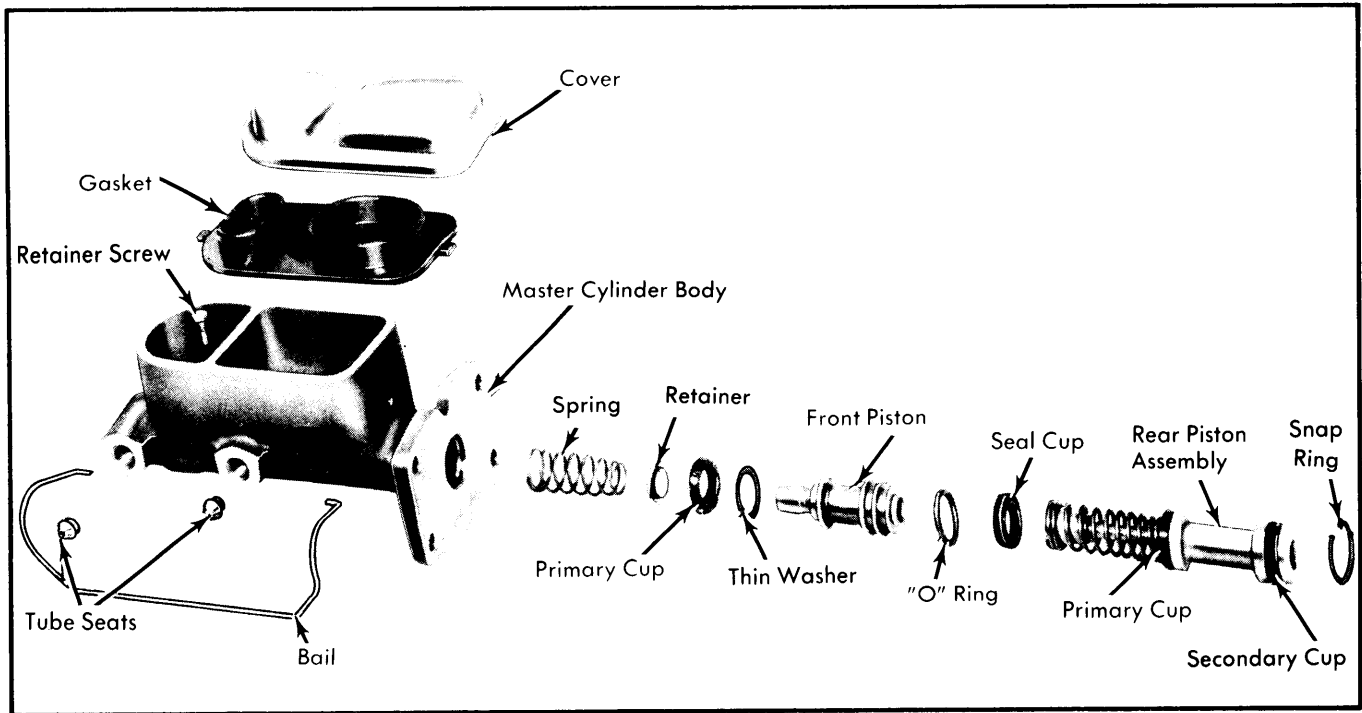
Fig. 3 Exploded View of Master Cylinder Assembly
