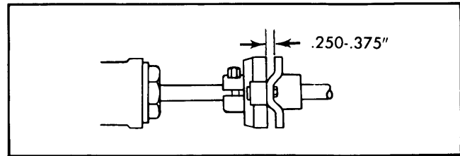
Fig. 6 Adjusting Flexible Coupling for All General Motors Models
