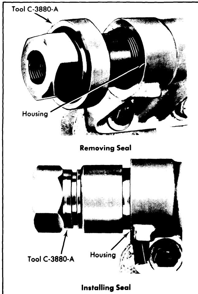
Fig. 7 Replacing the Sector Shaft Seal on Chrysler "B" and "PB" Models
