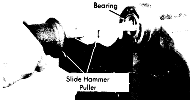
Fig. 9 Removing Wormshaft Bearing Race on Horizontal Sector Shaft Gear
