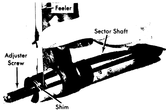
Fig. 12 Checking Lash Adjuster Clearance
