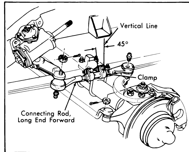
Fig. 4 "K" Models Steering Linkage
