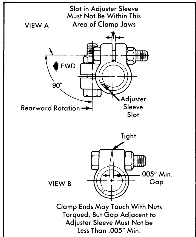
Fig. 7 Tie Rod Clamp Position "G" Models
