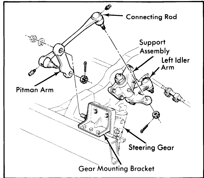
Fig. 3 "P" Models Motor Home Chassis Steering Linkage
