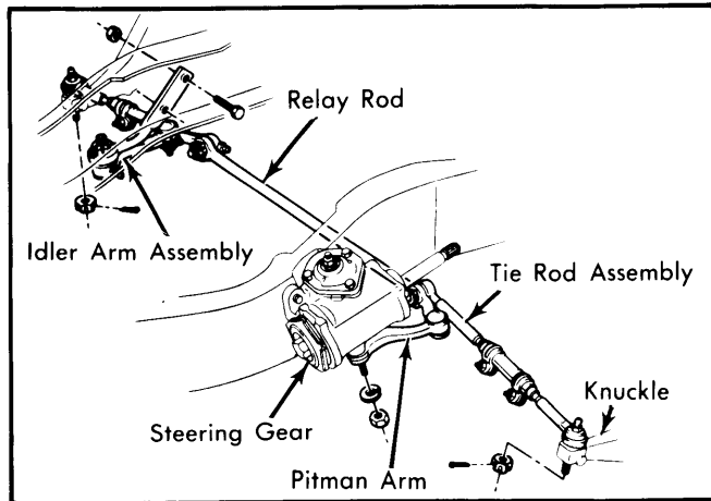
Fig. 1 "C" Models Steering Linkage
