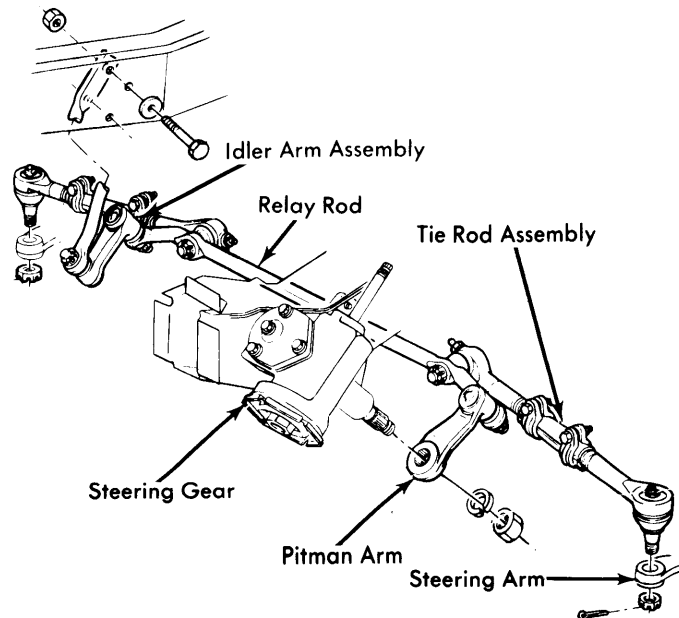
Fig. 2 "G" Models Steering Linkage
