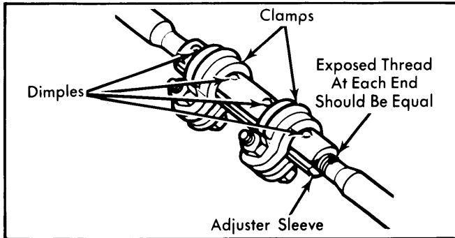
Fig. 5 Tie Rod Clamps Between Dimples (Typical)
