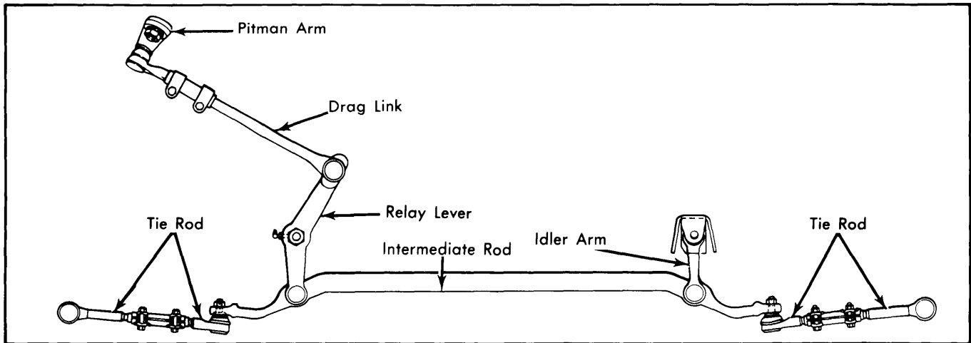
Fig. 9 GMC Motor Home Steering Linkage
