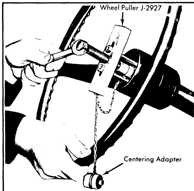
Fig. 3 Removing Steering Wheel using a Puller
