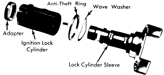
Fig. 9 Disassembled Lock Cylinder Assembly
