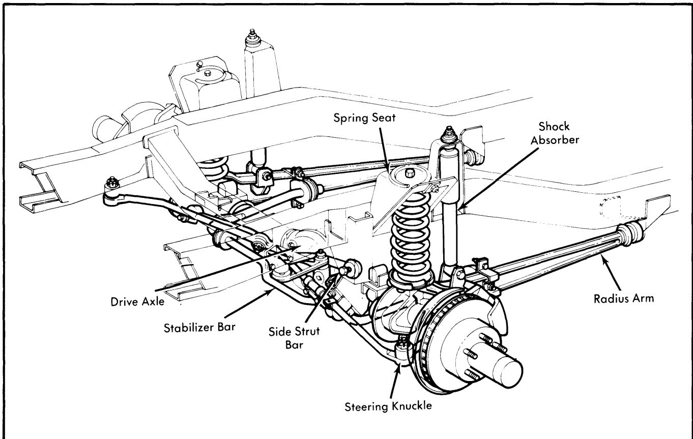
Fig. 1 U-100 (Bronco) Front Suspension Assembly F-150 Similar
