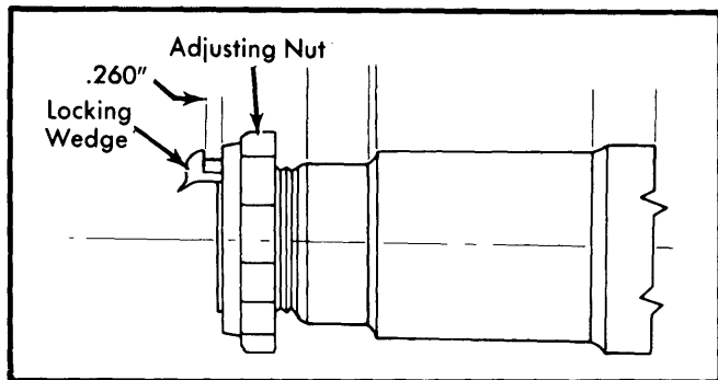
Fig. 1 Installing Locking Wedge Ford E250 and E350 Models
