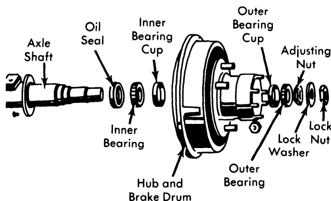
Fig. 2 Typical Full-Floating Rear Wheel Bearing
