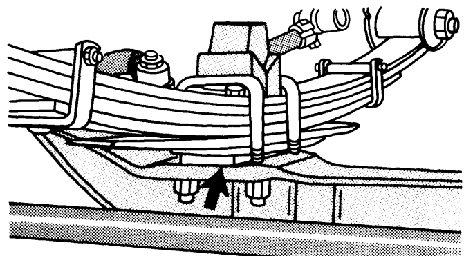
Fig. 1 Caster Adjustment
