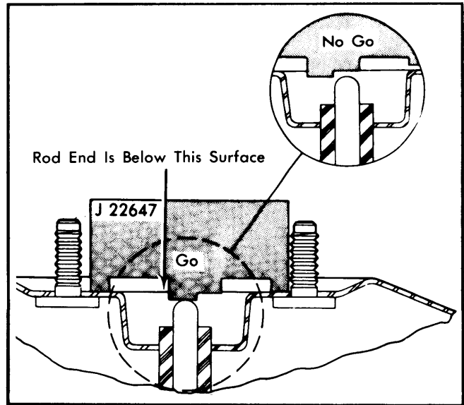
Fig. 2 Checking Piston Rod Height (Nonadjustable Rod Shown)
