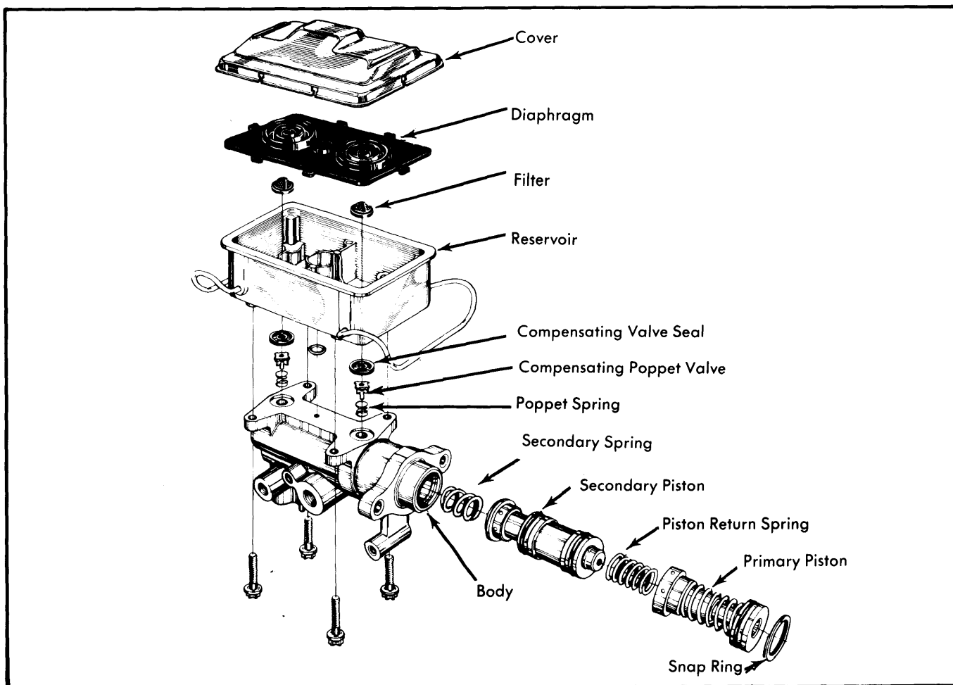
Fig. 1 Exploded View of Bendix Mini-Master Cylinder Assembly
