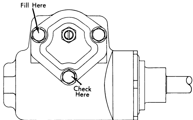
Fig. 3 Lubrication Check and Fill Holes for Gears without a Housing Plug
