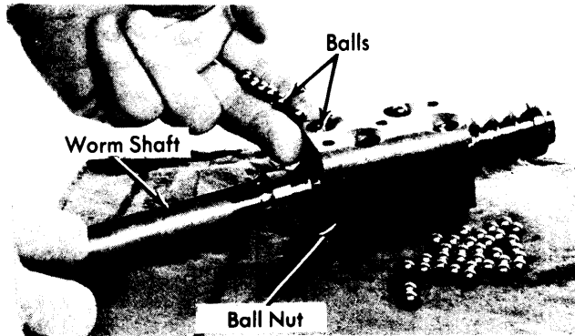
Fig. 11 Filling Ball Circuits Through Holes in Ball Nut
