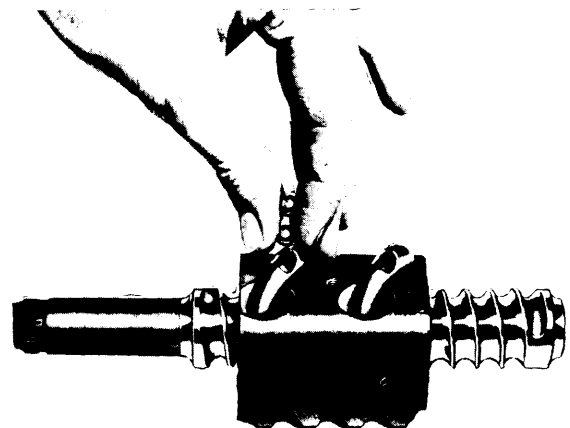
Fig. 10 Filling Ball Circuits Through Holes in Ball Guides
