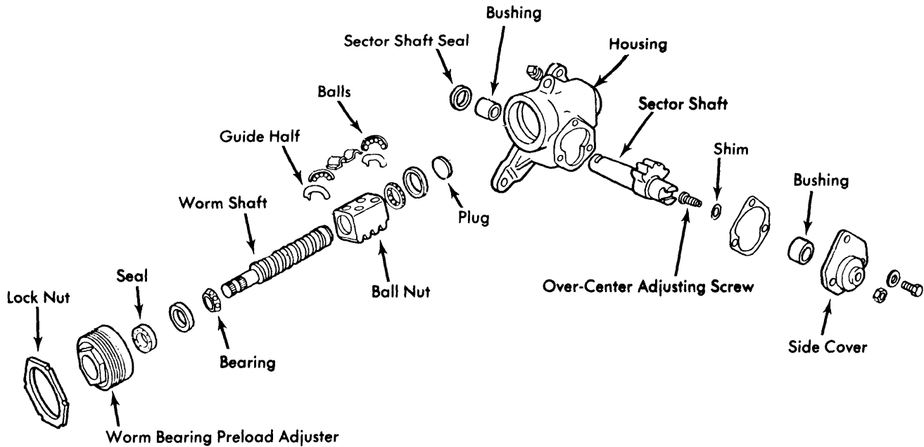
Fig. 8 Exploded View of Recirculating Ball Steering Gear (Chrysler Corp. "D" Model is Shown)
