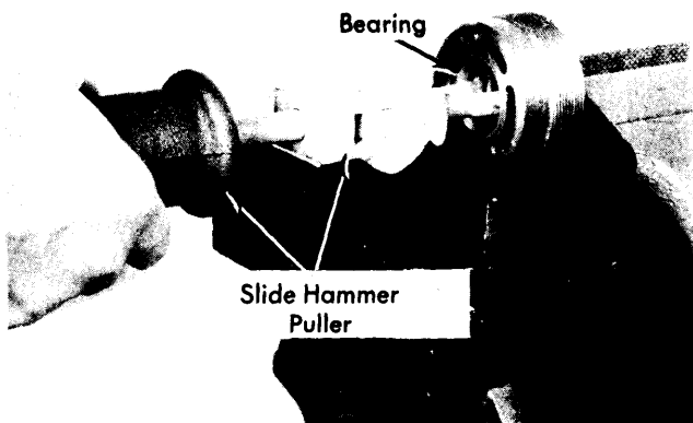
Fig. 9 Removing Wormshaft Bearing Race on Horizontal Sector Shaft Gear
