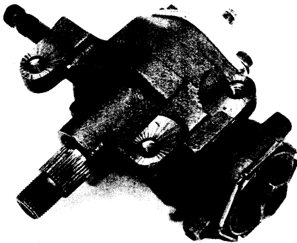
Fig. 1 Horizontal Sector Shaft Model of Saginaw Recirculating Ball Type Steering Gear
