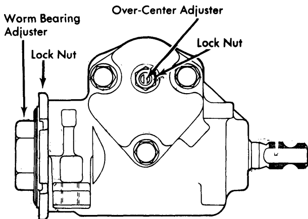
Fig. 4 Adjustment Points for Steering Gear
