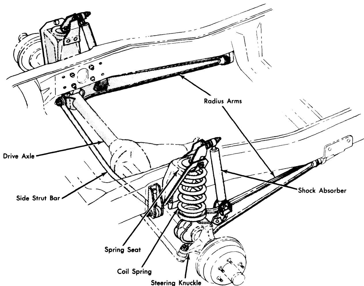
Fig. 1 Front Suspension Assembly
