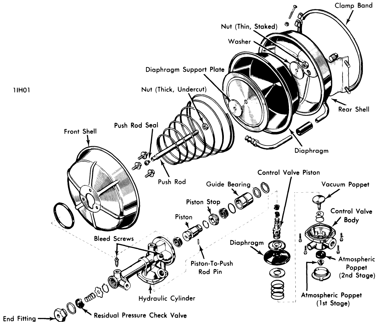
Fig. 1 Exploded View of Hydrovac Power Unit Assembly (Typical)
