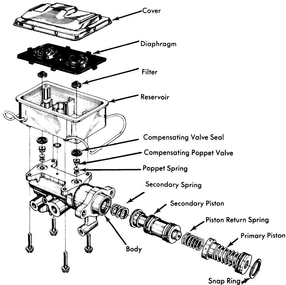
Fig. 1 Exploded View of Bendix Mini-Master Cylinder Assembly
