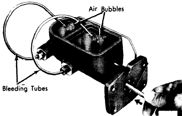
Fig. 2 Master Cylinder Bleeding Procedure
