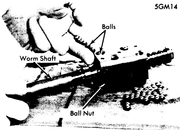
FILLING BALL CIRCUITS THROUGH HOLES IN BALL NUT
