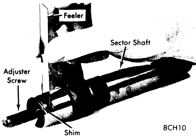
CHECKING LASH ADJUSTER CLEARANCE
