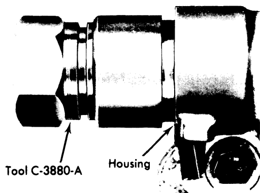
Installing Seal
