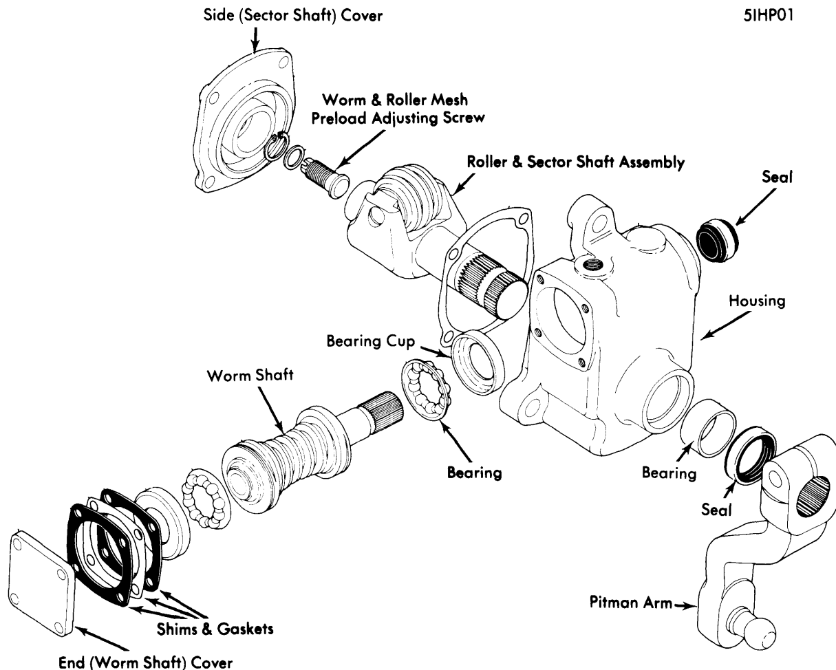
GEMMER/ROSS WORM & ROLLER STEERING GEAR ASSEMBLY
