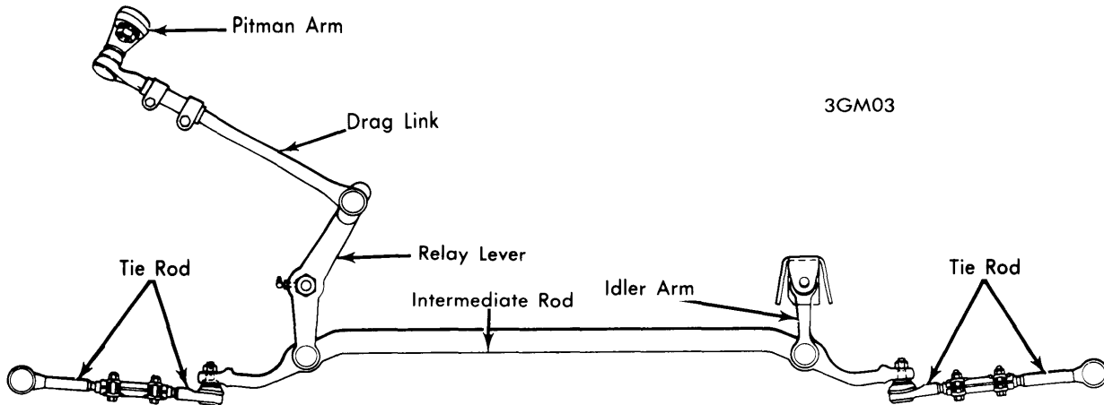
GMC MOTOR HOME STEERING LINKAGE
