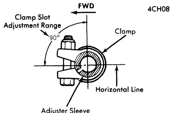
TIE ROD CLAMP POSITIONING, "G" MODELS
