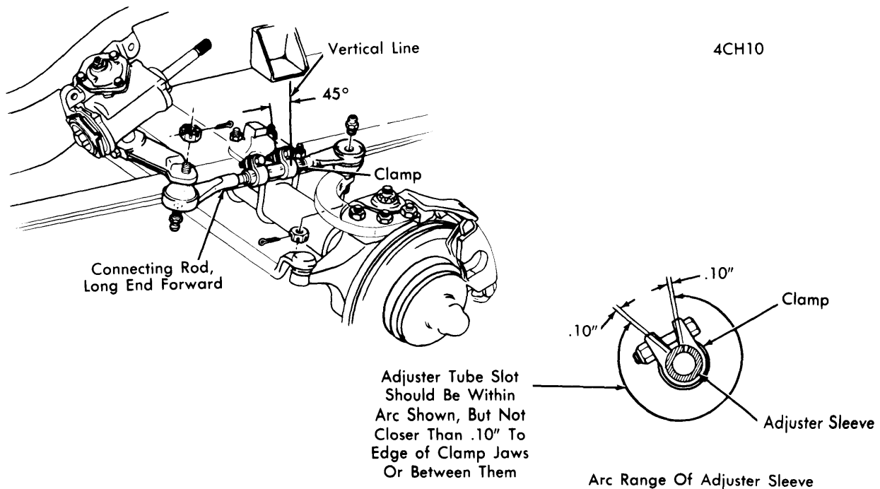
ADJUSTABLE CONNECTING ROD ASSEMBLY, "K" MODELS
