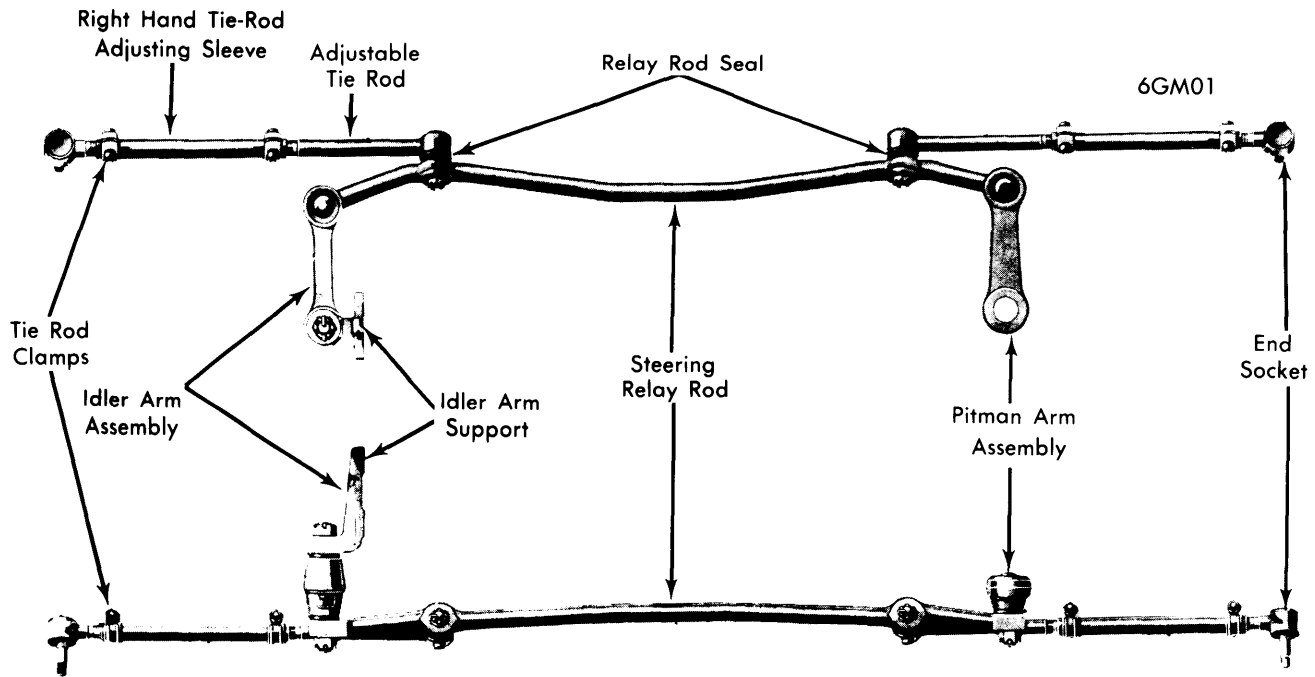
STEERING LINKAGE COMPONENTS, ALL MODELS WITH INDEPENDENT FRONT SUSPENSION
