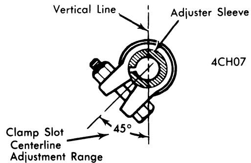
TIE ROD CLAMP POSITIONING, "C", "K" & "P" MODELS
