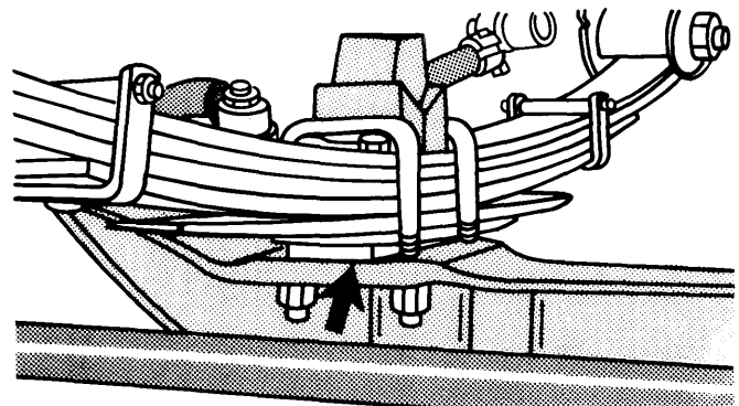
CASTER ADJUSTMENT
