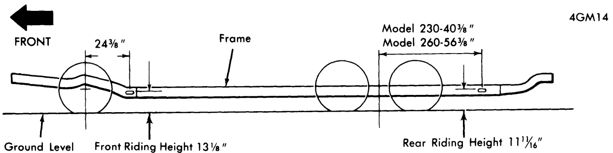
GMC MOTOR HOME RIDING HEIGHT
