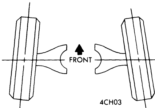
WHEEL TOE-IN
