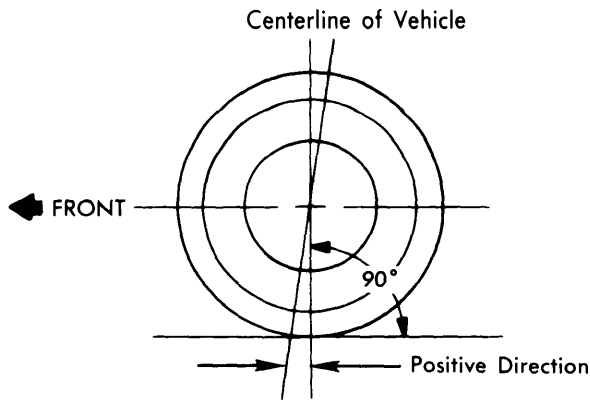
CASTER ANGLE
