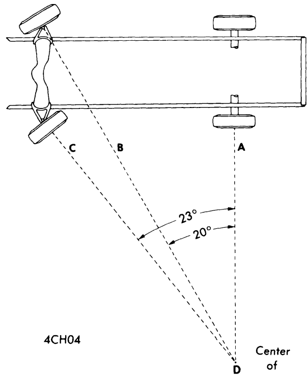
WHEEL TOE-OUT
