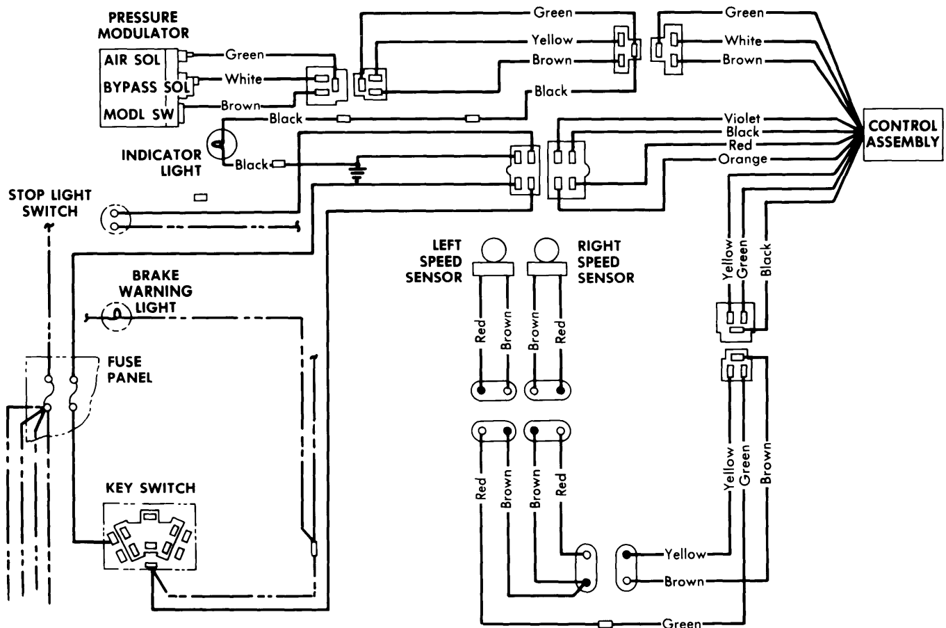
ELECTRIC CIRCUIT DIAGRAM
