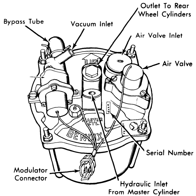
PRESSURE MODULATOR
