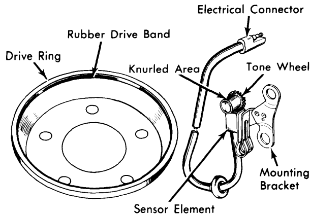
SPEED SENSOR DETAIL
