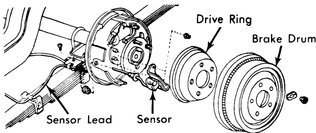
SPEED SENSOR MOUNTING
