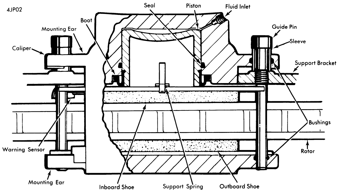
FLOATING CALIPER ASSEMBLY
