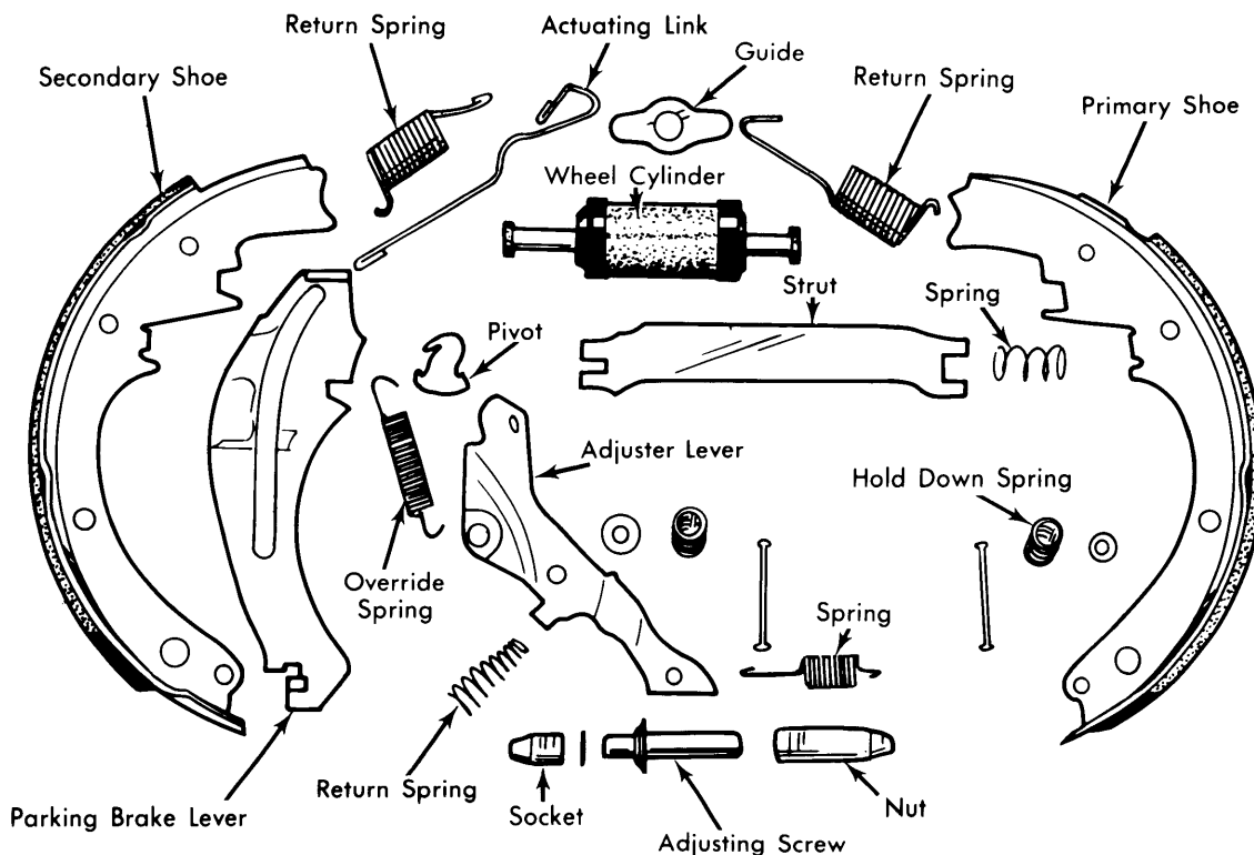
AUTOMATIC ADJUSTER BRAKE ASSEMBLY
