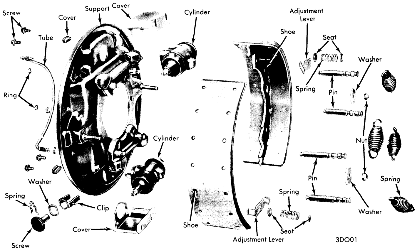
DUAL CYLINDER FLOATING SHOE BRAKE ASSEMBLY
