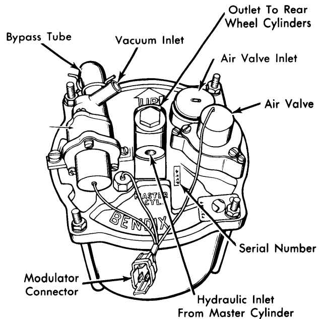
PRESSURE MODULATOR
