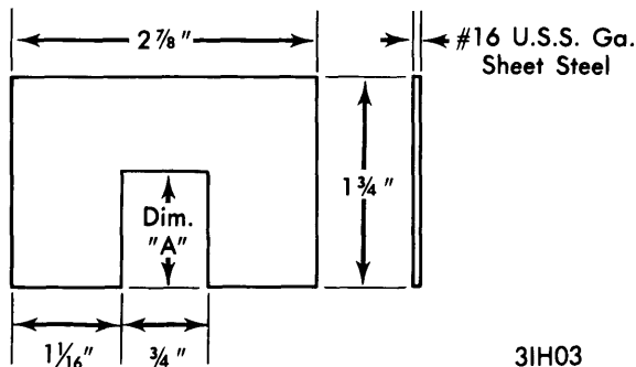
PUSH ROD GAUGE DIMENSIONS
