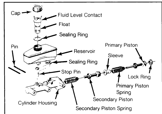
Fig. 5: Exploded View of Master Cylinder
