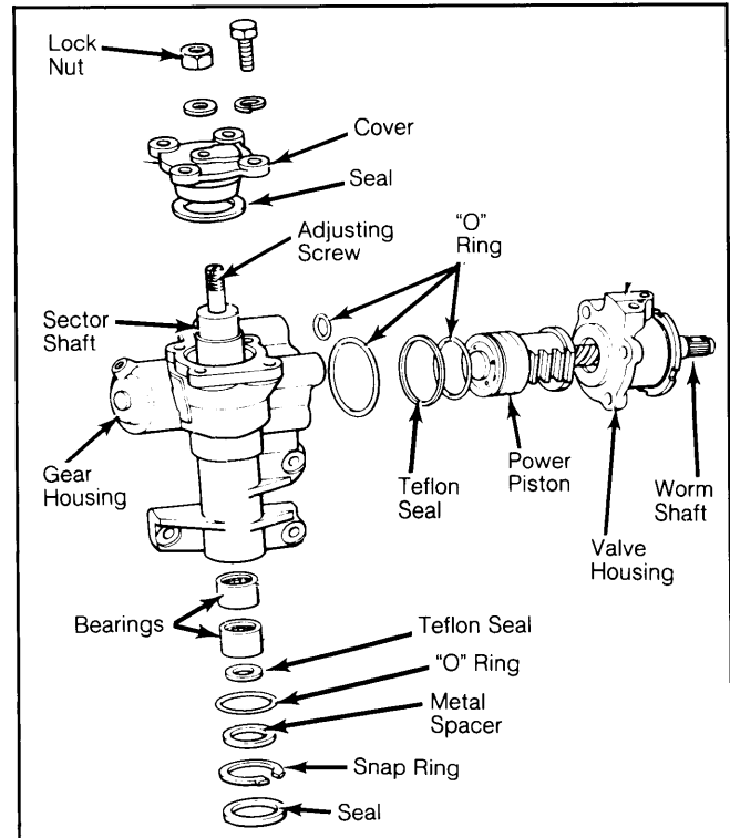
Fig. 4: Exploded View of Power Steering Gear Assembly
