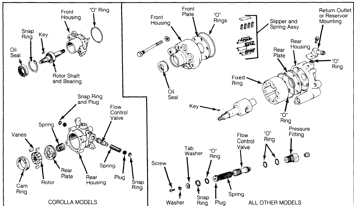
Fig. 1: Exploded View of Toyota Power Steering Pump Assemblies
