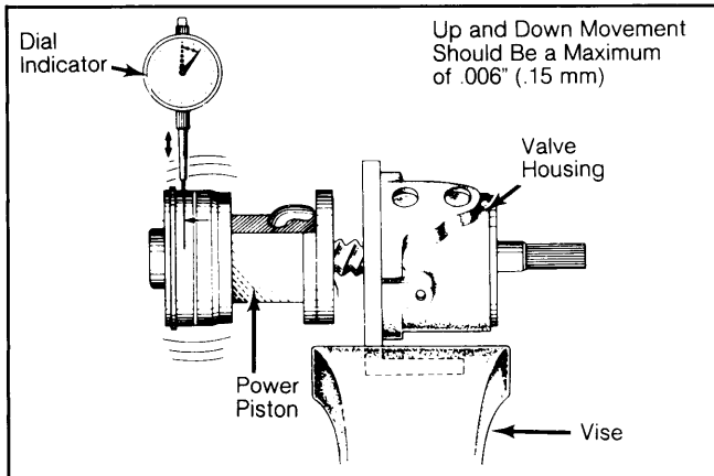
Fig. 2: Using Gauge to Check Ball Clearance
