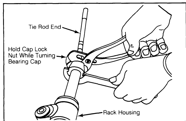
Fig. 2: Procedure for Removing Outer Bearing Cap Lock Nut
