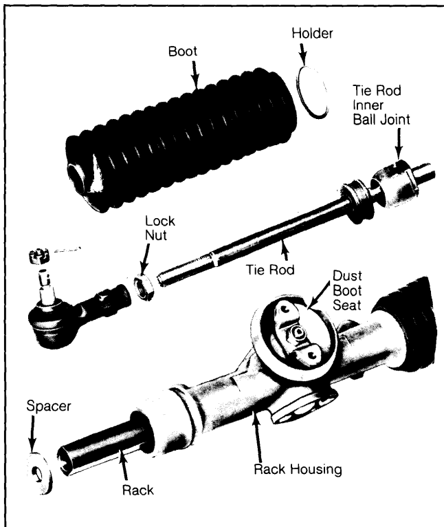
Fig. 3: Exploded View of 911SC Steering Gear Assembly
