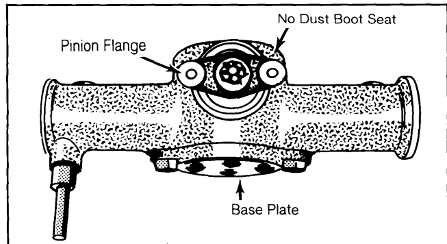
Fig. 2: Plastic Pressure Block Housing Assembly
