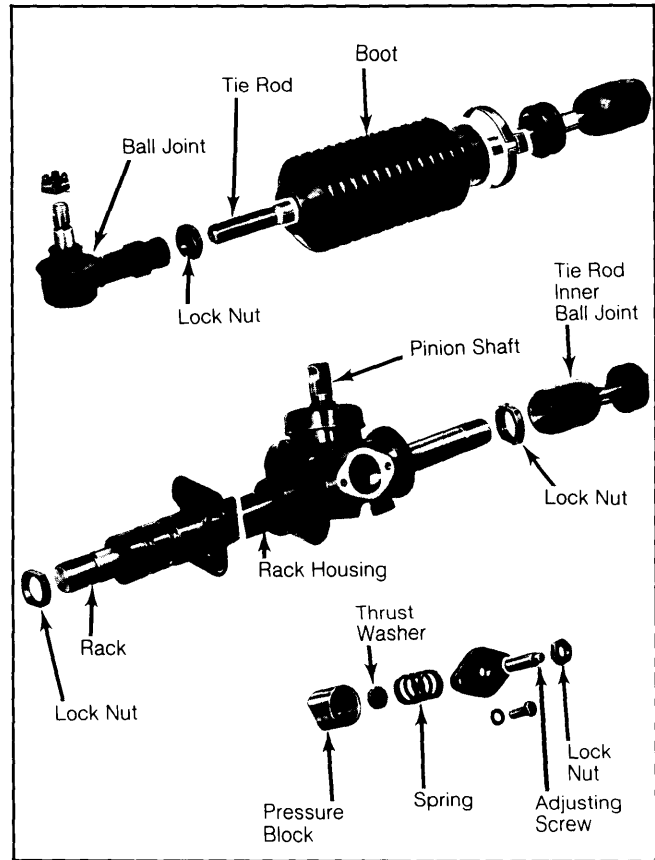
Fig. 4: Exploded View of Porsche 924 Steering Gear Assembly
