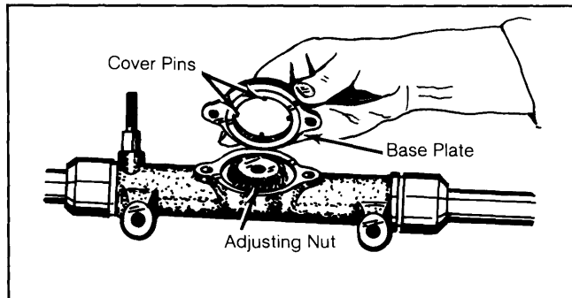
Fig. 1: Adjusting Nut with Cover
