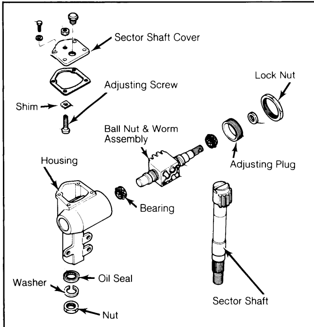
Fig. 2: Exploded View of Recirculating Ball Steering Gear Assembly (200SX & Pickup Models)
