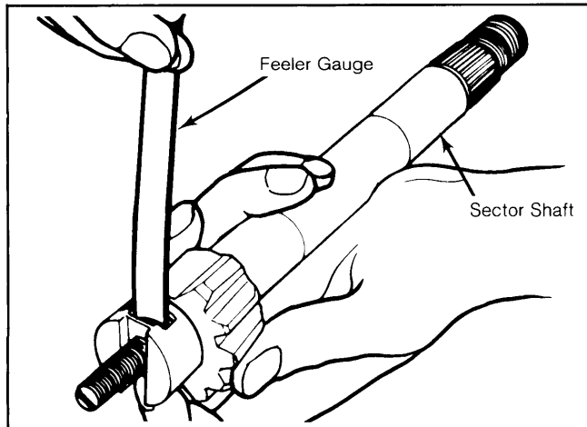
Fig. 5: Insert Feeler Gauge into Sector Shaft to Measure Sector Shaft-to-Adjusting Screw End Play
