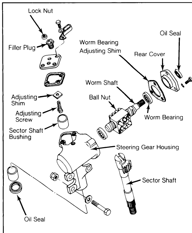
Fig. 3: Exploded View of Recirculating Ball Steering Gear Assembly (210 Model)
