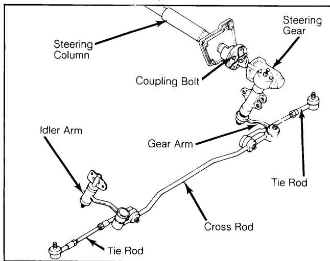
Fig. 1: Datsun Steering Gear Linkage (210 Shown, Others Similar)
