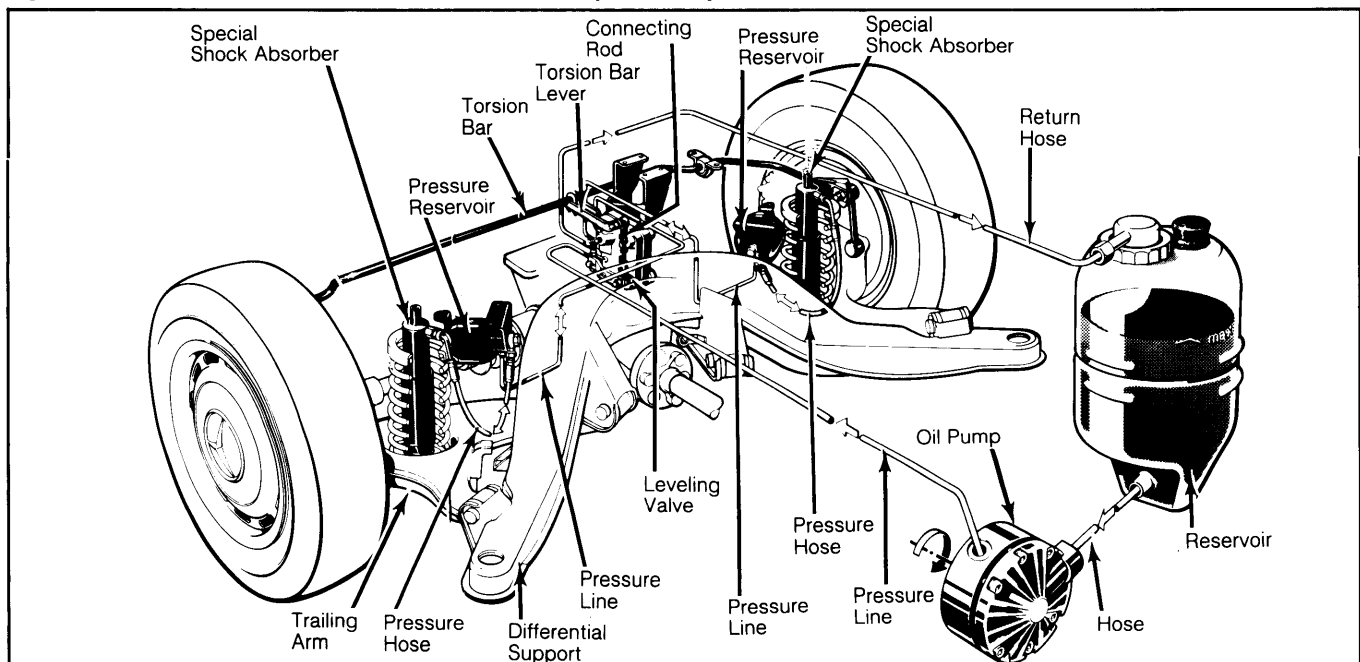
Fig. 1: Mercedes-Benz 300TD Level Control Rear Suspension System
