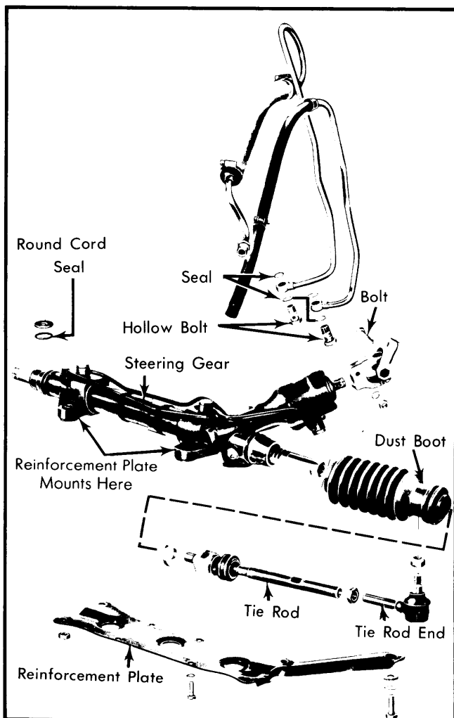
Fig. 1 Power Steering Gear Porsche 928
