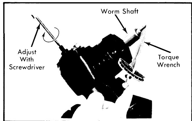
Fig. 5 Measuring Final Worm Bearing Preload
