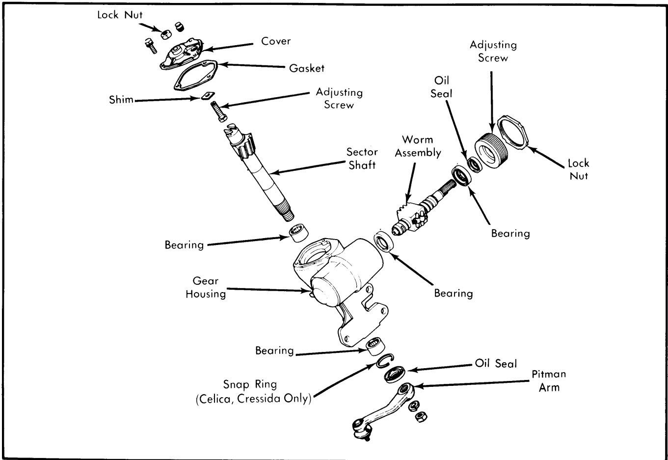
Fig. 3 Exploded View of Steering Gear Assembly (Except Pickup 4-WD)
