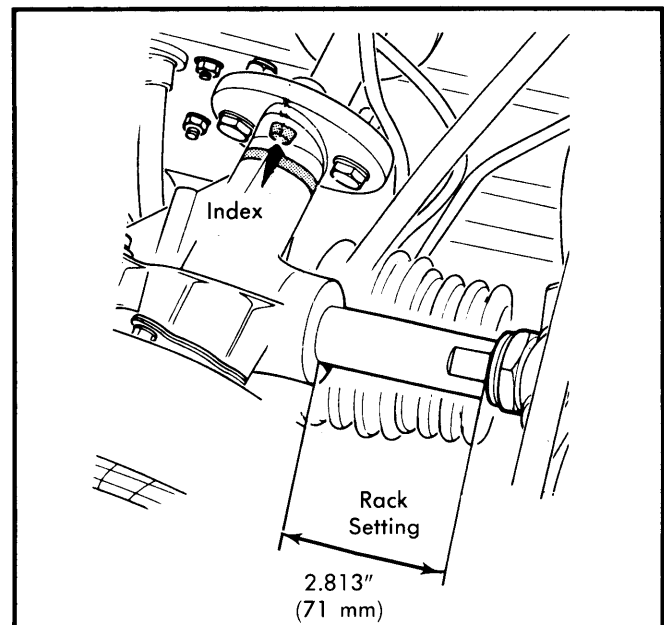
Fig. 3 Steering Center Measurement
