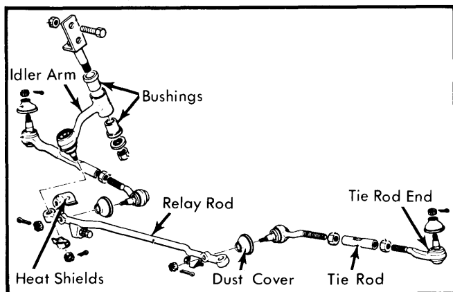
Fig. 1 Exploded View Showing Steering Linkage Components
