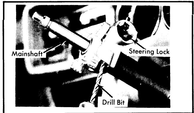
Fig. 3 Drilling Out Shear Head Bolt to Remove Steering Lock from Shaft
