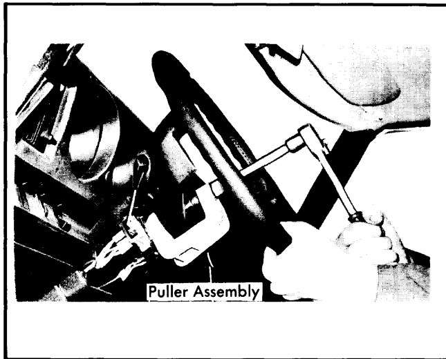
Fig. 1 Using Universal Puller Tool to Remove Steering Wheel Assembly
