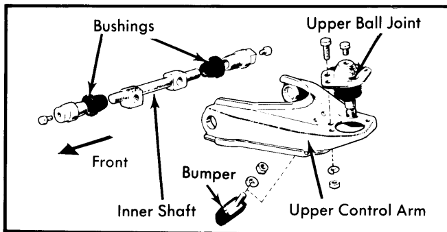
Fig. 2 Exploded View of Upper Control Arm Assembly
