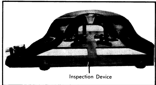
Fig. 4 Inspection Tool 115 589 04 23 00
