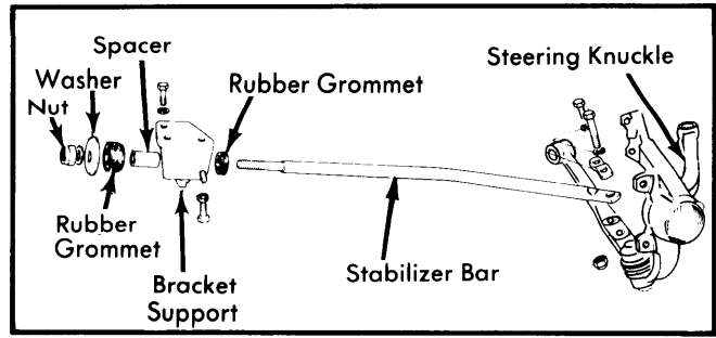
Fig. 3 Exploded View of Stabilizer Bar Assembly
